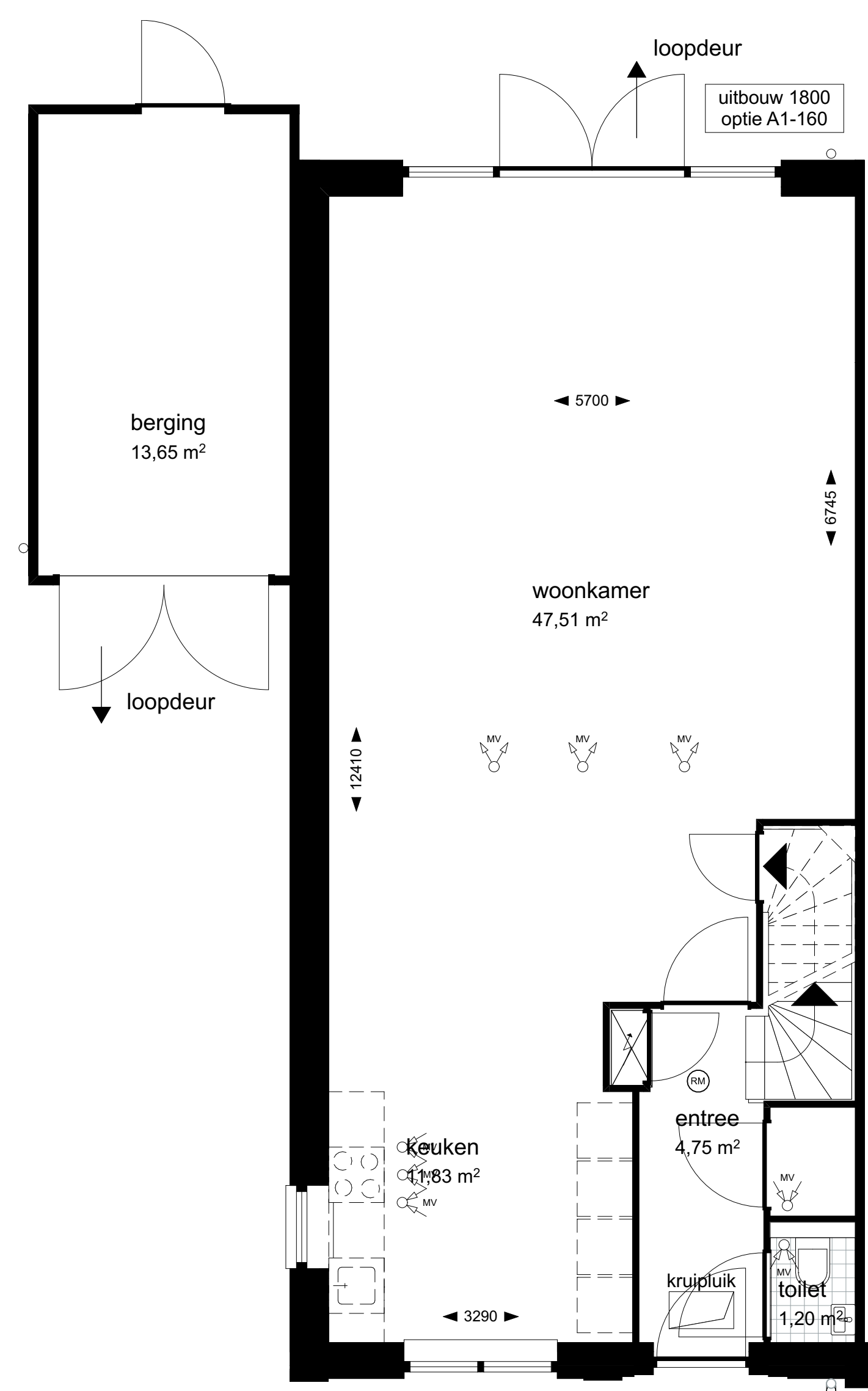
1:50 00 Begane grond
