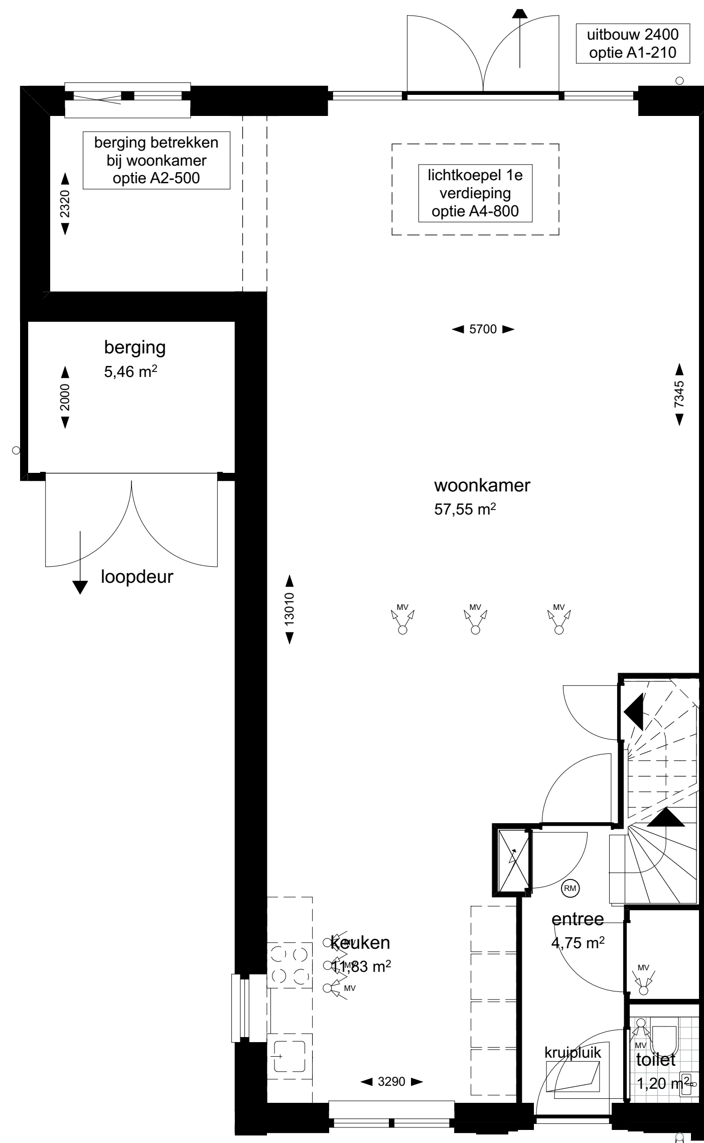
1:50 00 Begane grond
