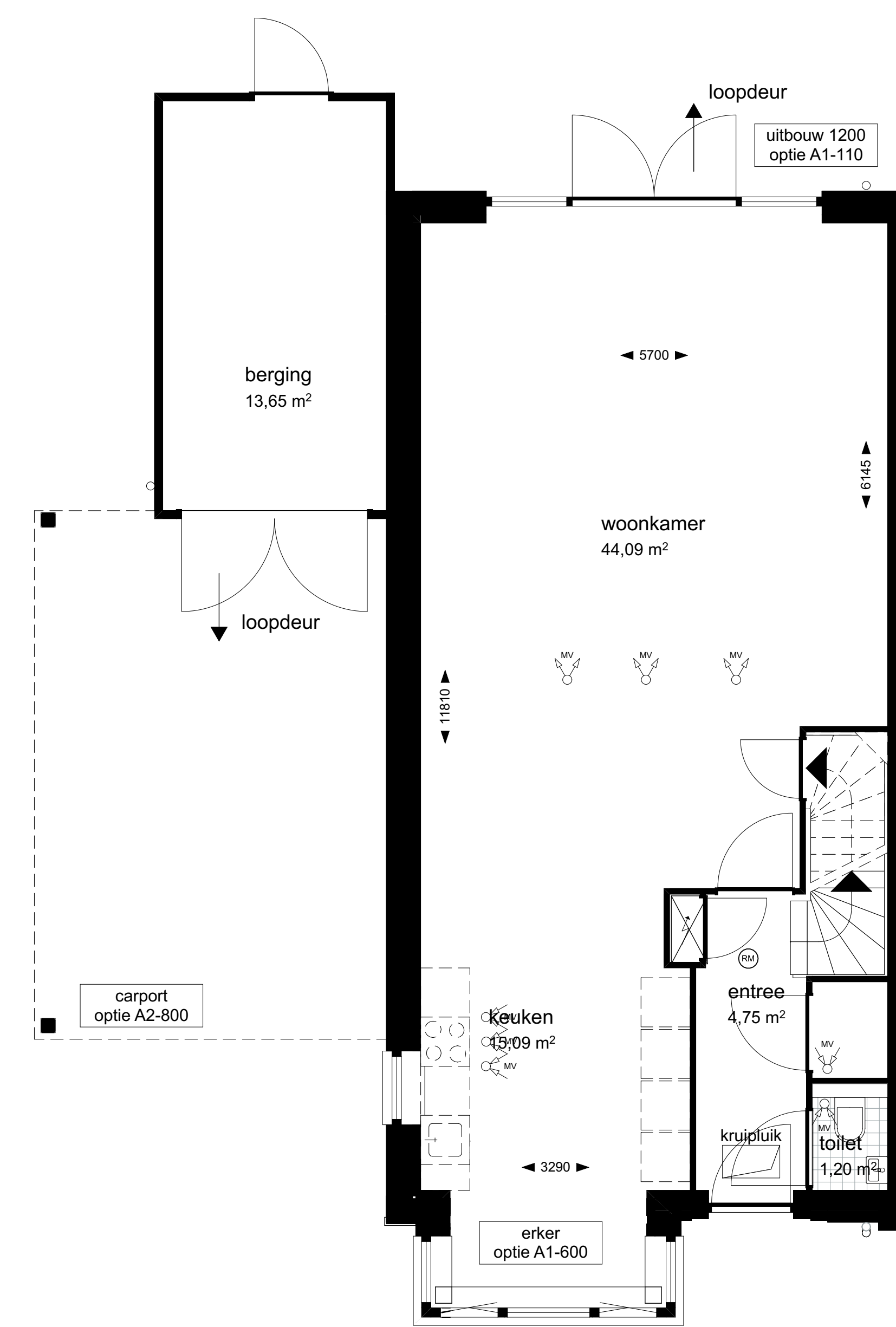
1:50 00 Begane grond
