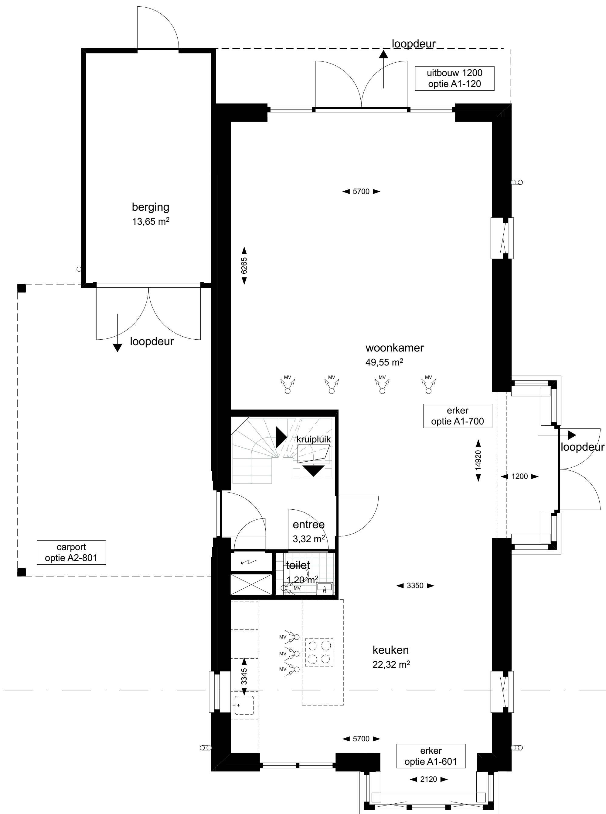
1:50 00 Begane grond
