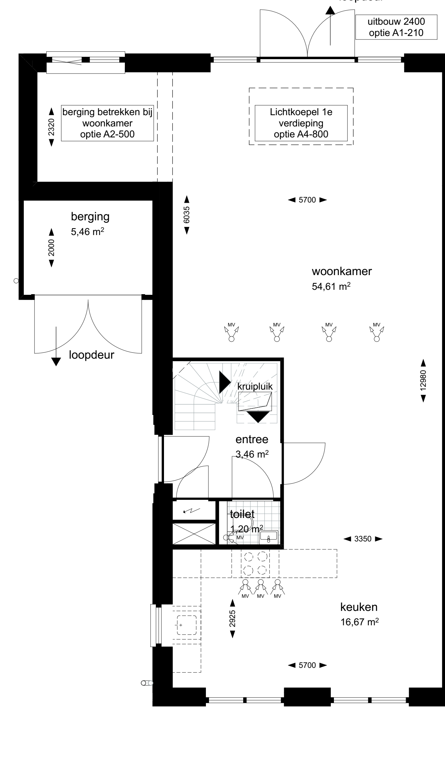
1:50 00 Begane grond
