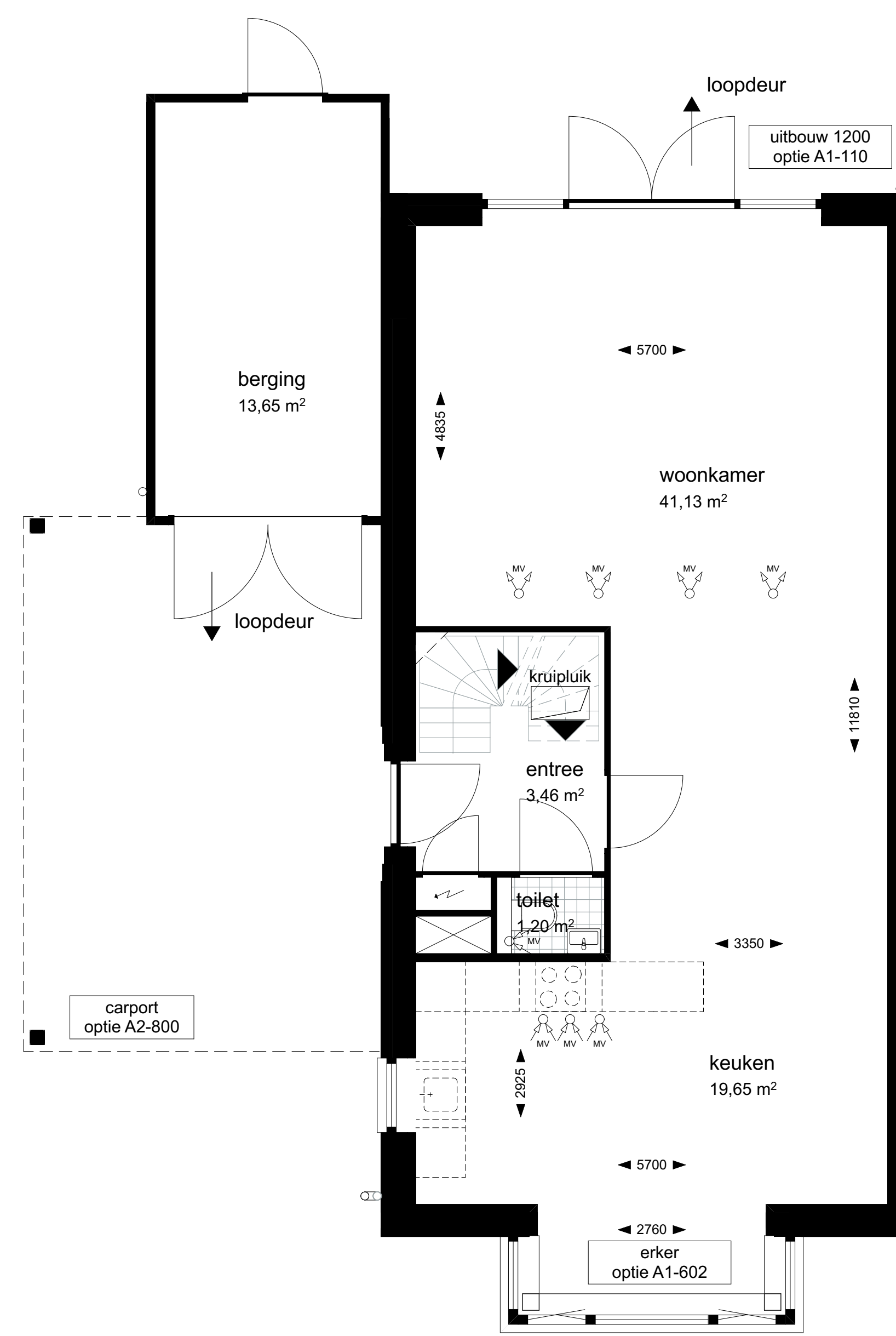
1:50 00 Begane grond
