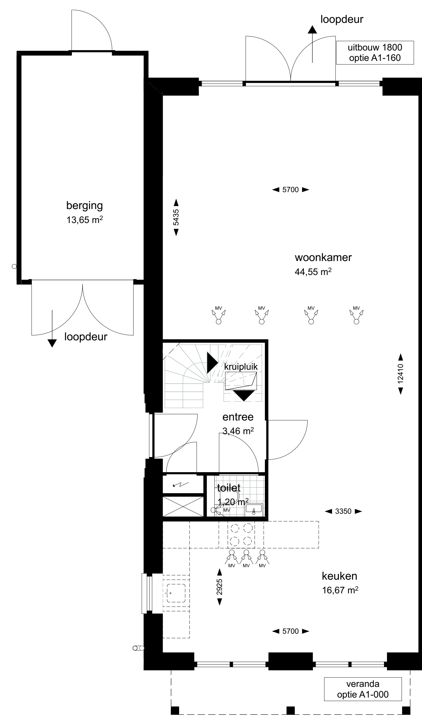
1:50 00 Begane grond
